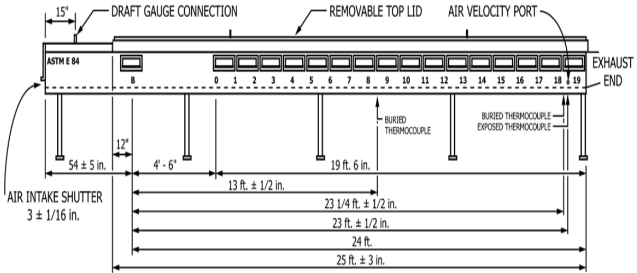
Diagram 1. Test Chamber side view showing critical dimensions.
