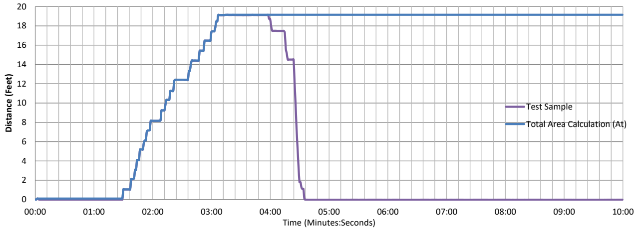
Smoke Readings
